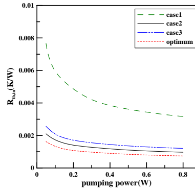
Fig. 7 Distribution of inlet thermal resistance at different pumping power
