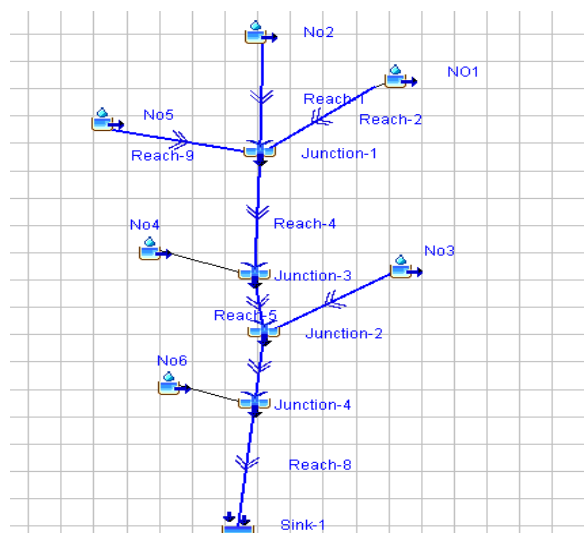
Fig. 2 Local Watershed DARBAND in HEC-HMS software
