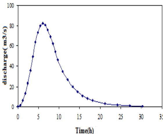
Fig. 3 Derived unit hydrograph of area by SCS method
