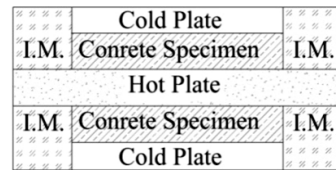
Fig. 3 Thermal conductivity test setup *I.M.: Insulation material
