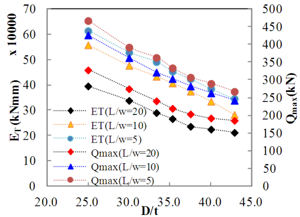
Fig. 11 Effect of diameter-to-thickness ratio and slit length-to-width ratio on maximum shear force and cumulative energy
