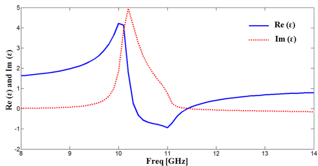
Fig. 5 Constitutive Permittivity of ETDS
