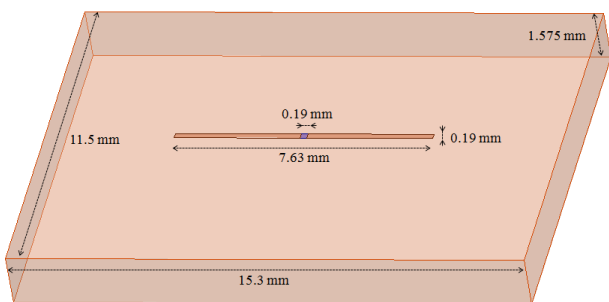
Fig. 2 Small Planar Dipole Antenna (SPDA)
