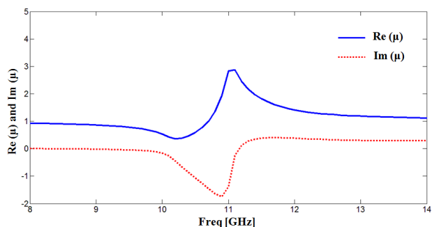
Fig. 6 Constitutive Permeability of ETDS
