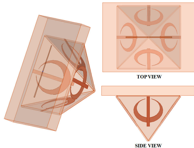
Fig. 1 Small Planar Dipole Antenna (SPDA) mounted on a Symmetrical Pyramidal Block (SPB)
