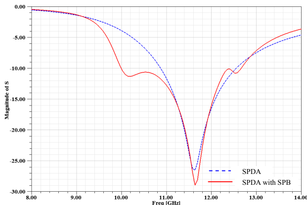
Fig. 7 The Reflection Coefficient of SPDA and SPDA with SPB
