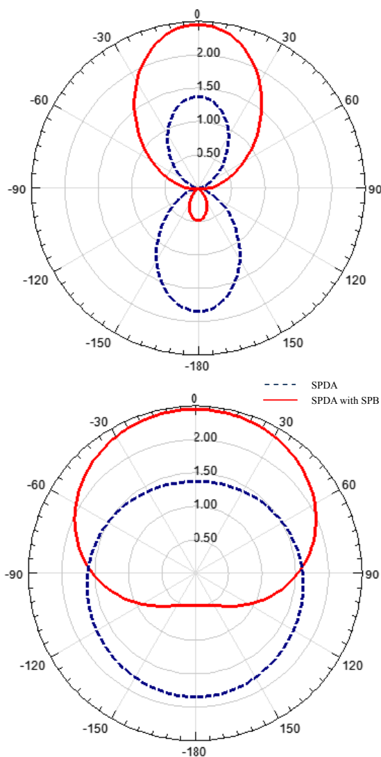
Fig. 8 The Radiation Pattern of the SPDA and the SPDA with SPB
