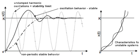
Fig. 2 Example of stable system transfer function
