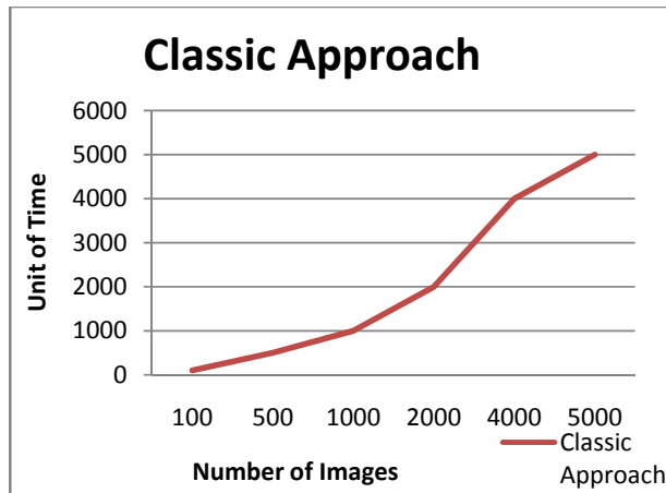
Fig. 7 Time Complexity Analysis for Classic Approach
