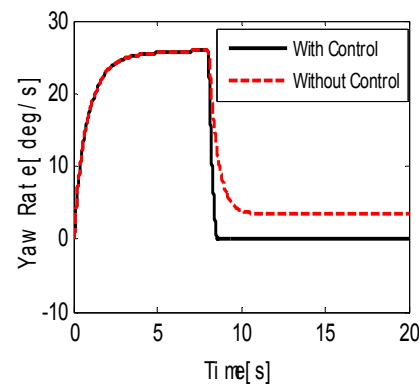
Fig. 14 Yaw rate at 30km/h
