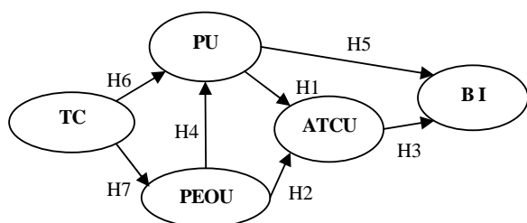
Fig. 1 Research model
