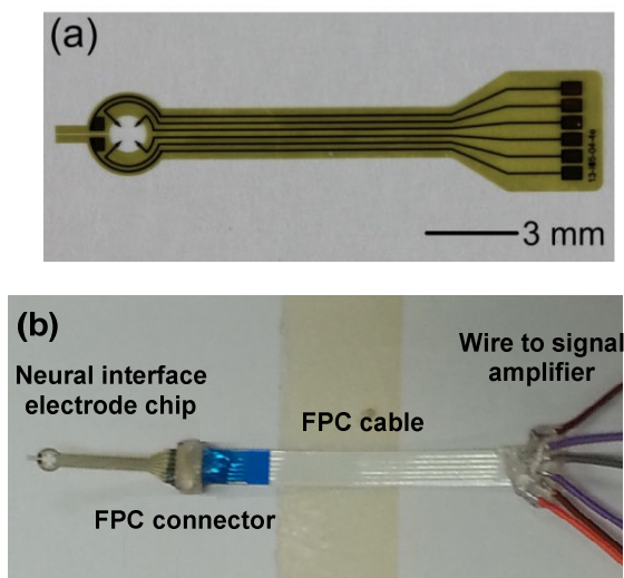
Fig. 3 (a) Photography of released chip, (b) packaged device
