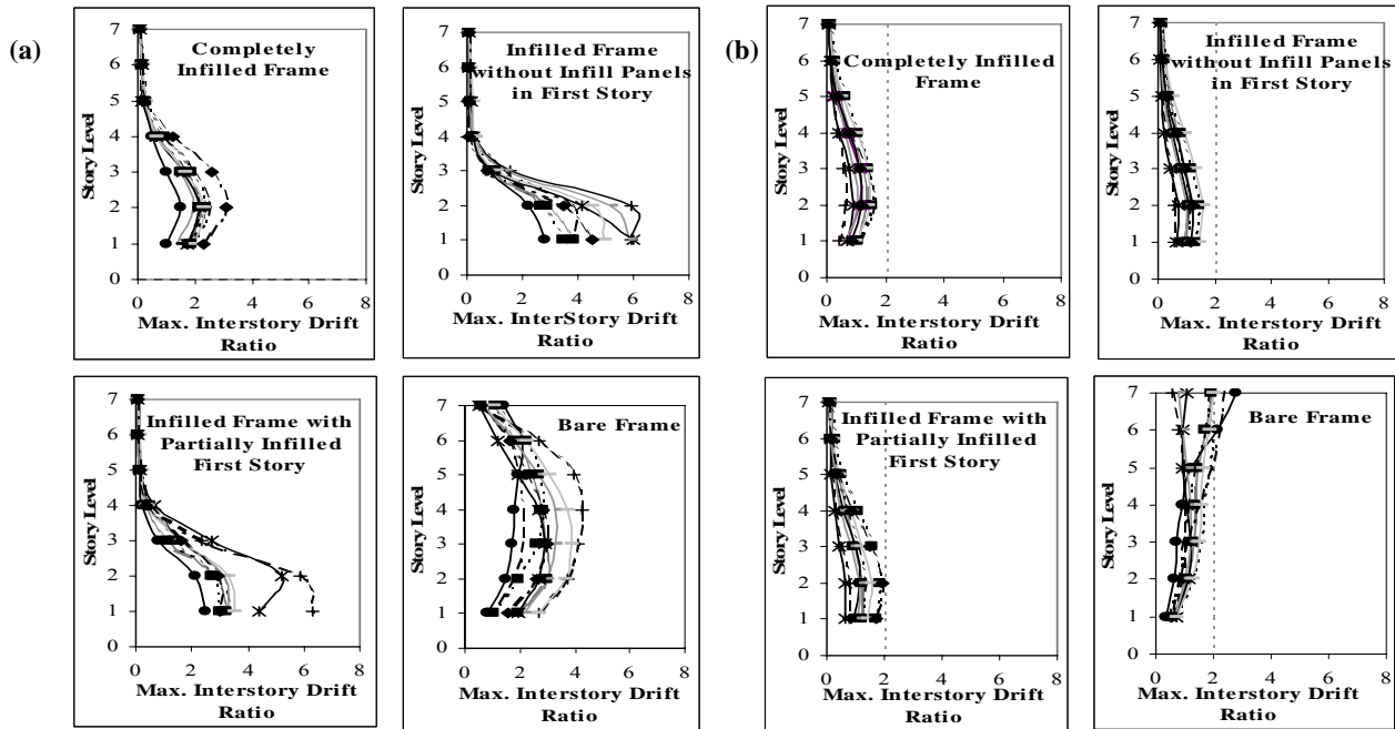
Fig. 4 Peak Normalized Inter-Story Drifts (%) of the R/C Frame Designed using (a) Code Specified Force Based Design Procedure and (b) Energy Based Plastic Design Procedure for Target Drift of 2%
