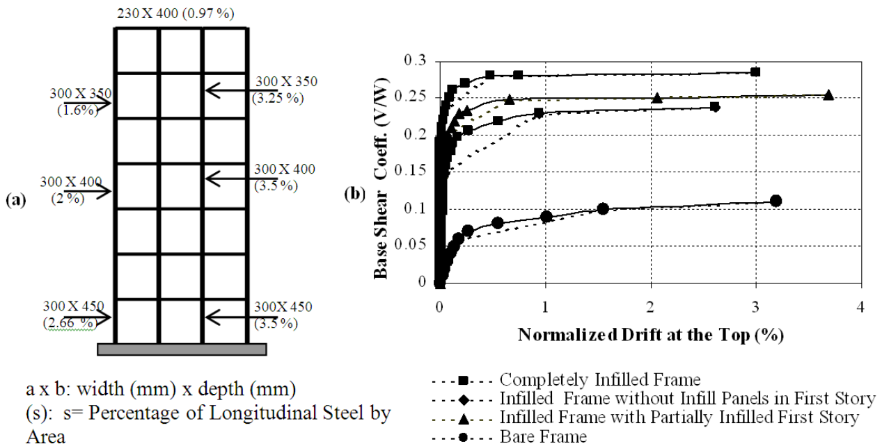
Fig. 2 Design Dimensions and Details and Capacity Curves of Code Compliant R/C Frame: (a) Dimensions and Reinforcement Details of the Code-Compliant R/C Frame and (b) Capacity Curves for the Code-Compliant Masonry Infilled R/C Frames
