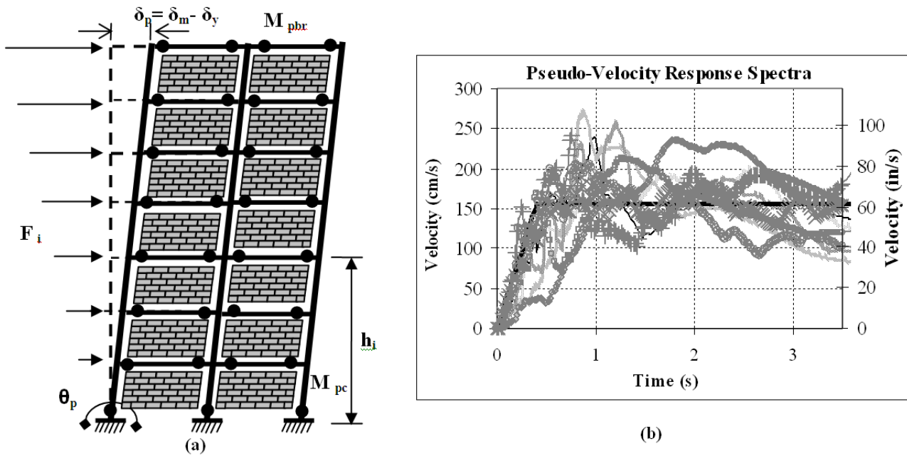
Fig. 1 Key Components of the Energy Balance Concept: (a) Multi bay Frame with selected Global Plastic Mechanism and (b) Pseudo-Velocity Response Spectra of the Scaled Earthquake Ground Motion Records and Design Response Spectrum
