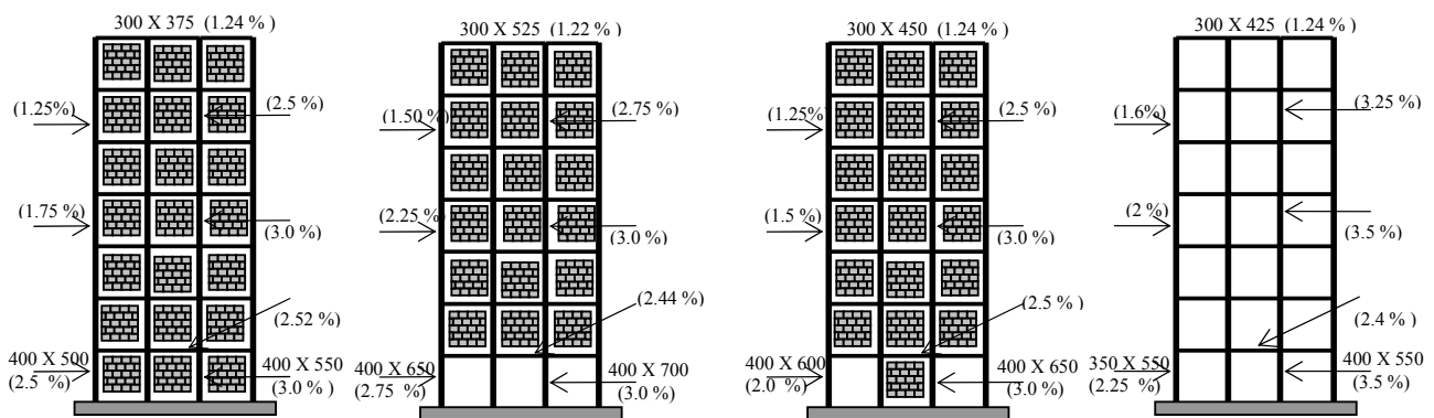
Fig. 3 Dimensions and Reinforcement Details of the R/C Frame designed by Energy Based Approach for Target Drift of 2%
