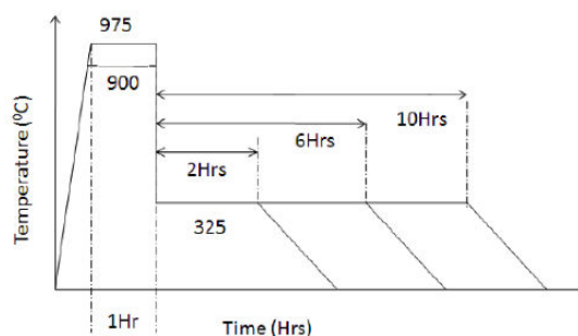
Fig. 1 Schematic representation of austempering treatment employed
