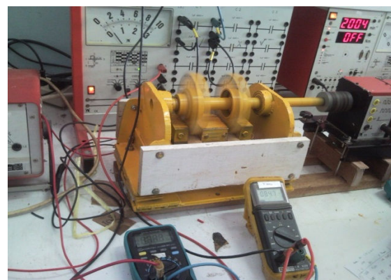
Fig. 14 Permanent magnet reluctance generator prototype new designs trials
