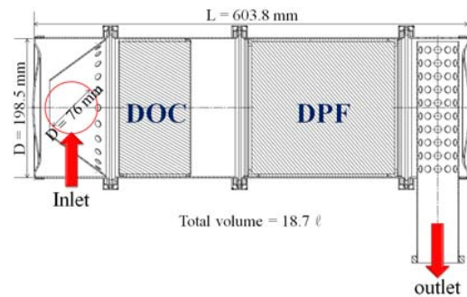
Fig. 1 Catalytic muffler adopted in this work
