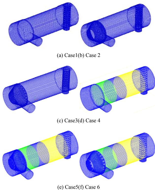
Fig. 2 Computational grid system of the catalytic muffler
