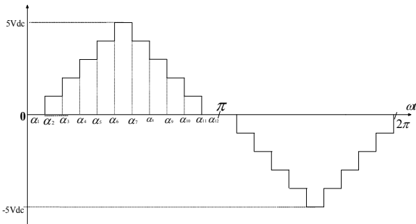
Fig. 1 Multilevel inverter waveform
