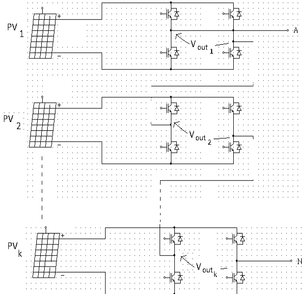
Fig. 1 Single Phase n - level Structure of Cascaded H-Bridge Inverter
