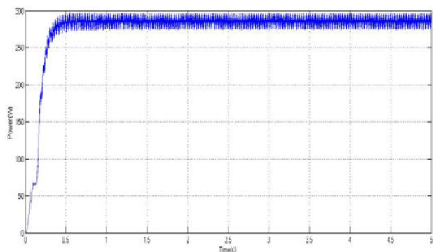
Fig. 10 Output Power Waveform of Hill-Climbing Algorithm
