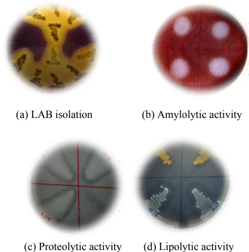
Fig. 1 (a) Isolation of LAB on MRS agar supplemented with bromocresol purple and \text{CaCO}_3 . (b) Amyolytic activity on starch agar. (c) Proteolytic activity on skim milk agar. (d) Lipolytic activity on tributyrin agar
