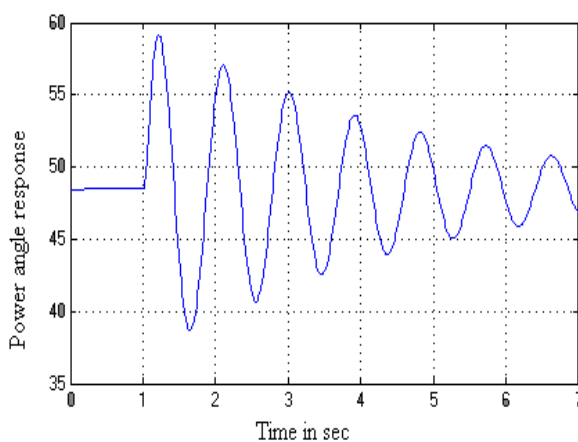
Fig. 11 Power angle response without SSSC Controller
