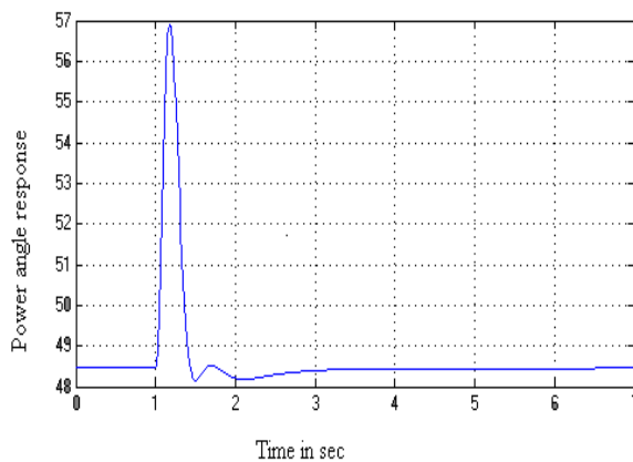
Fig. 12 Power angle response with SSSC Controller
