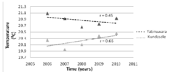
Fig. 3 Trend of change in mean annual minimum air temperatures during 2006 – 2010
