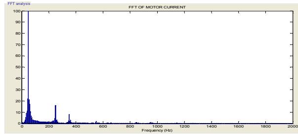
Fig. 14 FFT for simulated motor current
