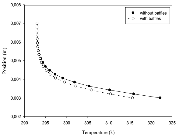
Fig. 9 Temperature profiles ( x= 10\text{ mm} )
