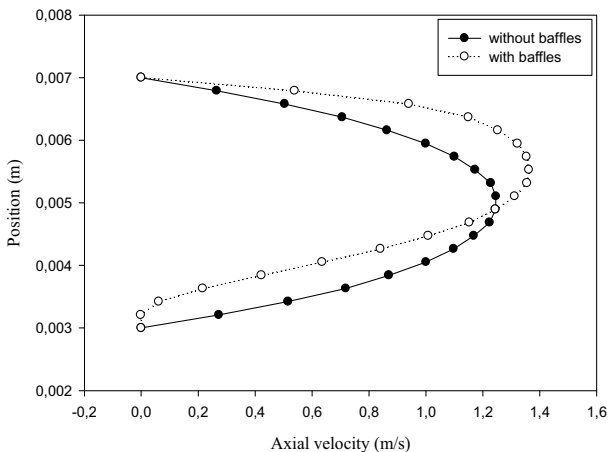
Fig. 8 Axial velocity profiles ( x= 61\text{ mm} )
