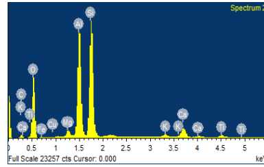
Fig. 3 EDAX of Ground Bottom Ash
