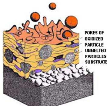
Fig. 2 The scheme of thermal coating structure [1]
