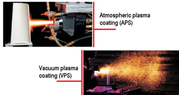
Fig. 4 Plasma coatings [8]
