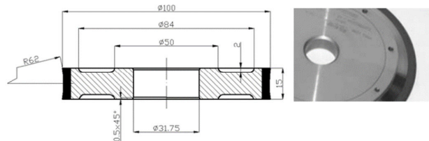
Fig. 6 The grinding wheel 1FF1V 100 – 15 – R62 – 31.75 D126 Ni [9]
