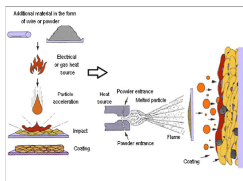
Fig. 1 The scheme of thermal coating [1]
