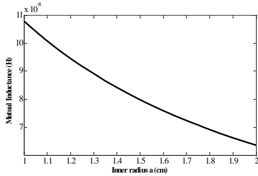
Fig. 3 Mutual inductance for circular core Rogowski coil with respect to inner radius, with N=100 turns
