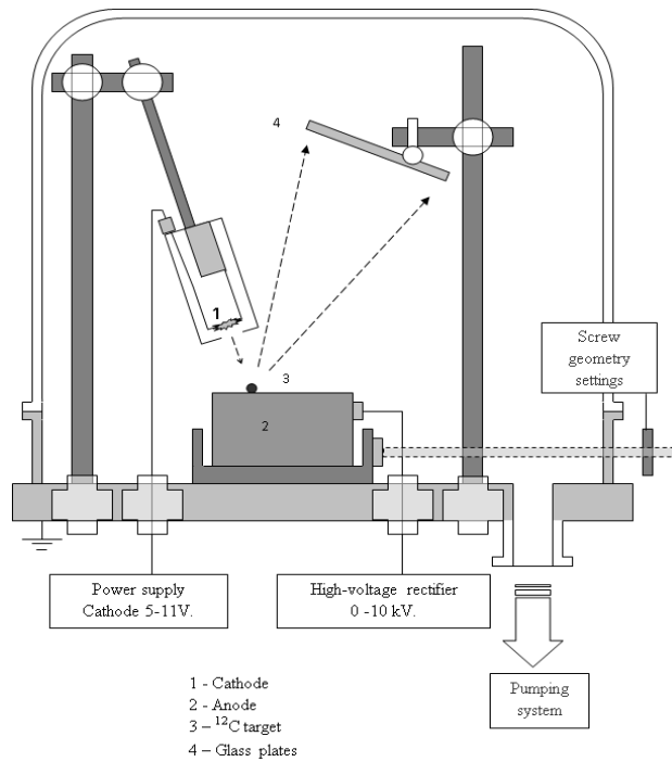
Fig. 2 Block diagram for the device used for the deposition of ^{12}\text{C} on glass plates using electron gun
