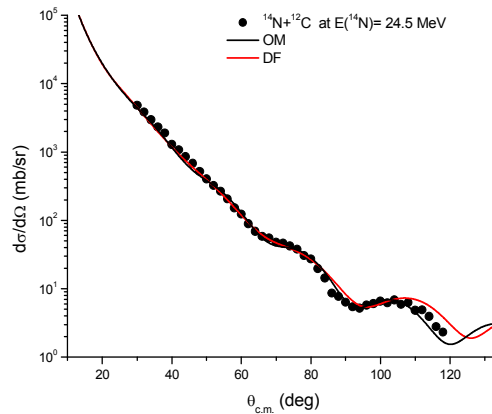
Fig. 7 Same as Fig. 5 but for energy 24.5 MeV
