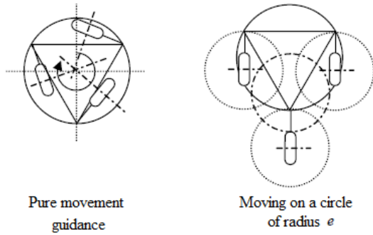
Fig. 6 Movements decoupling the actuators
