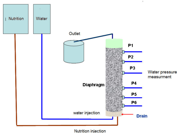
Fig. 2 Experimental device
