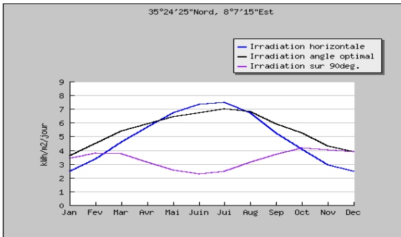
Fig. 17 The solar irradiance received on a horizontal plane at an optimum angle and 90 ° for Ferkene [17]
