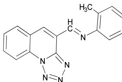
Fig. 1 (E)-2-methyl-N-(tetrazolo[1,5-a]quinolin-4-ylmethylene)aniline (QMA)
