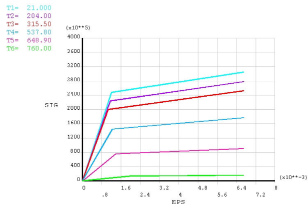
Fig. 2 Elasto-plastic stress-strain
