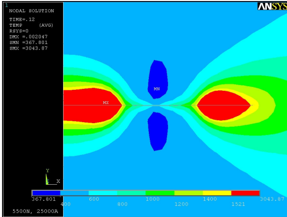
Fig. 8 Crack welding
