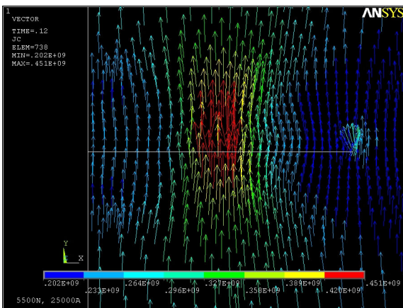
Fig. 9 Electrical contact
