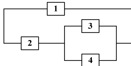
Fig. 1 4-Unit system
