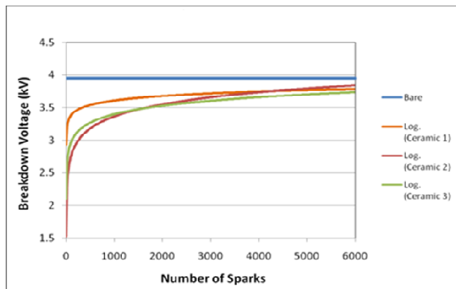
Fig. 11 Durability of MWCNT/ceramic mix over 6000 sparks
