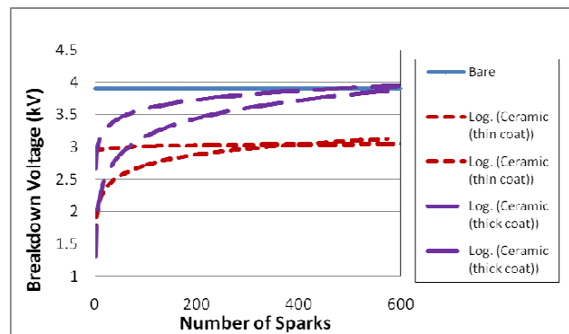
Fig. 10 Durability of MWCNT/ceramic mix
