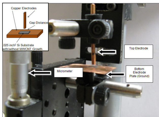
Fig. 4 Copper electrodes and micrometer stage
