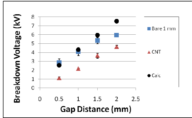
Fig. 7 Breakdown voltage vs. gap distance
