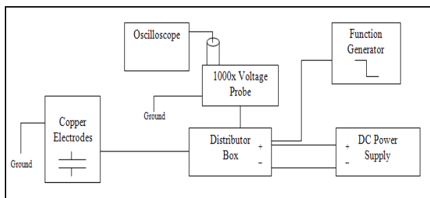
Fig. 3 Breakdown voltage testing schematic
