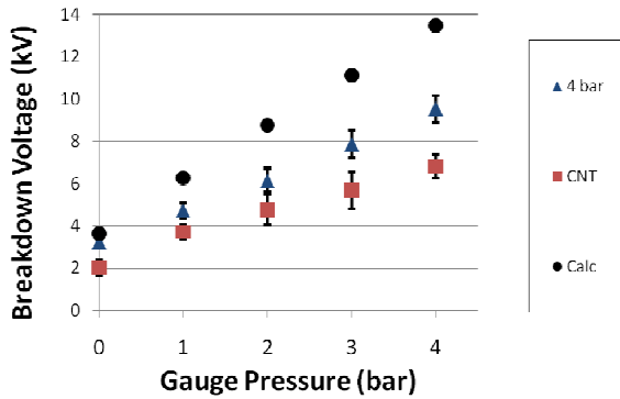
Fig. 8 Breakdown voltage vs. gauge pressure (1mm gap)
