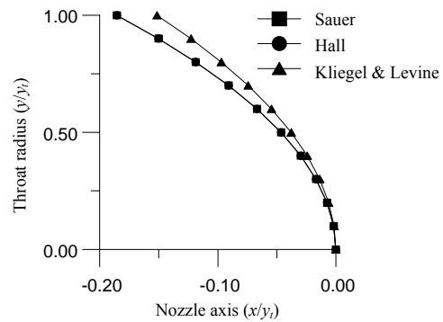
Fig. 2 Sonic lines for Nozzle 2
