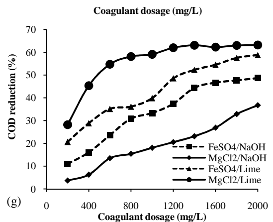
Fig. 2 Effect of coagulant dosage on the COD reduction for synthetic textile wastewater containing (a) RB5 (b) CR (c) DB3 (d) RB5+CR (e) CR+DB3 (f) RB5+DB3 (g) RB5+CR+DB3
