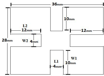
Fig. 1 Top view of Slotted Patch Antenna
