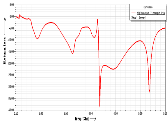
Fig. 9 Return Loss (in dB) vs. freq (in GHz) for slotted patch antenna with directly coupled parasitic elements and embedded fractal EBG structures
