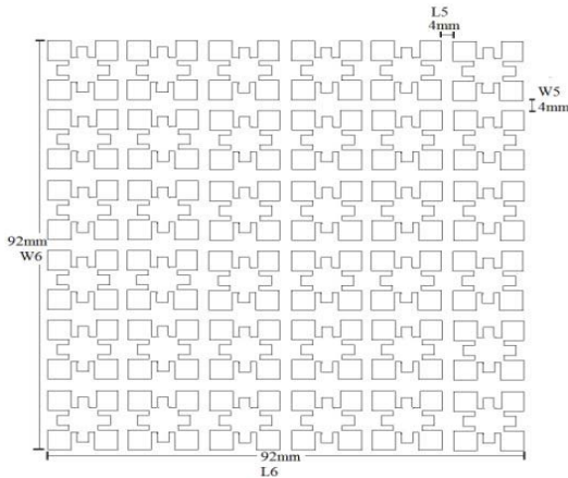
Fig. 5 6×6 array of EBG structures
