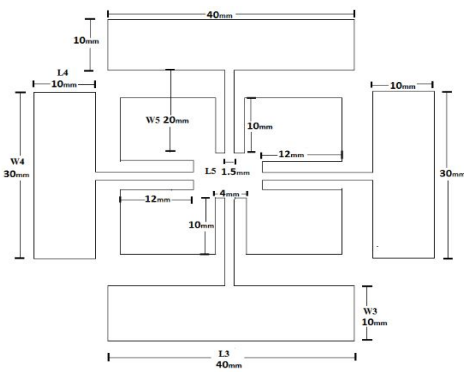
Fig. 2 Top view of Slotted Patch Antenna with directly coupled parasitic elements
