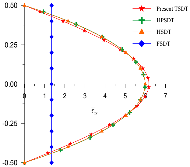
Fig. 9 Variation of transverse shear stress ( \bar{\tau}_{zx} ) through the thickness of simply supported beam at ( x = 0, z ) when subjected to cosine load and obtain using constitutive relation for aspect ratio 10 (Example 1)
