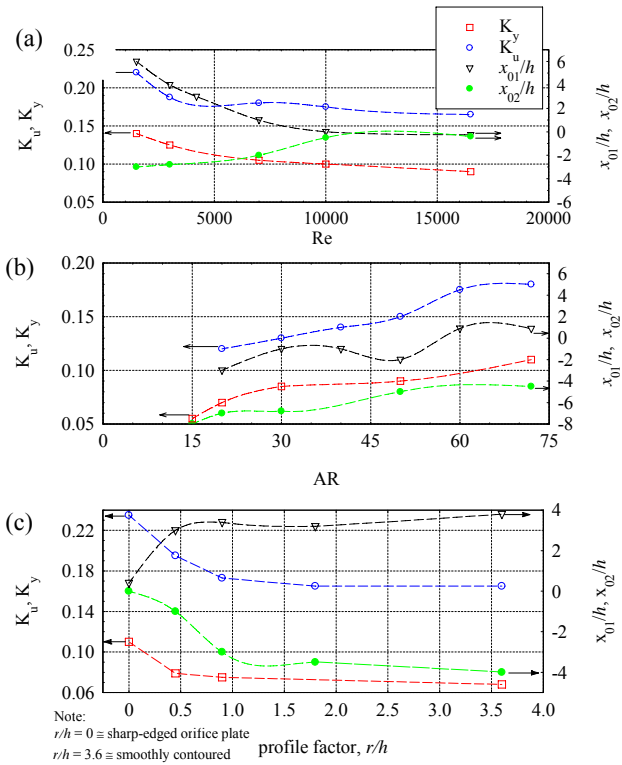
Fig. 3 Effect of nozzle-exit conditions on decay rate ( K_u ) and virtual origin ( x_{01}/h ) based on axial velocity profiles, jet spreading date ( K_y ) and virtual origin ( x_{02}/h ) based on lateral velocity profiles. (a) Re = 1500 - 16500 ( AR = 60, r^* = 2.1 ), (b) AR = 15 - 72 ( Re = 18\,000, r^* = 3.60 ), (c) r^* = 0 - 3.60 ( Re = 18\,000, AR = 72 ) (Redrawn after [10], part (a); [8], part (b); [7], part (c))
