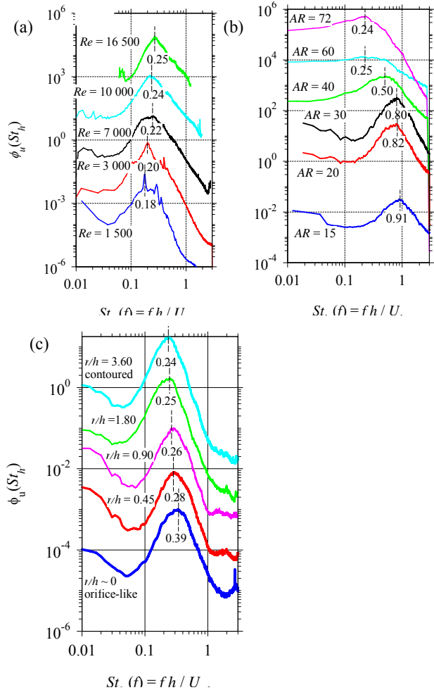
Fig. 10 The power spectral density \Phi_u(St_h) versus Strouhal number St_h = fh / U_h representing the evolution of primary eddy structures at x/h = 3 for (a) Re = 1500 - 16500 ( AR = 60, r^* = 2.1 ), (b) AR = 15 - 72 ( Re = 18000, r^* = 3.60 ), (c) r^* = 0 - 3.60 ( Re = 18000, AR = 72 )
