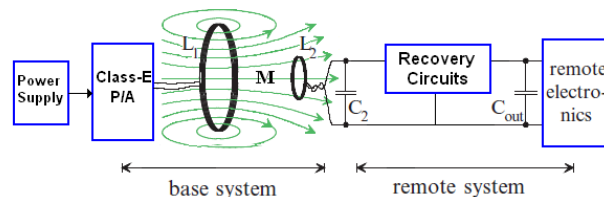
Fig. 1 Inductive power transmission block
