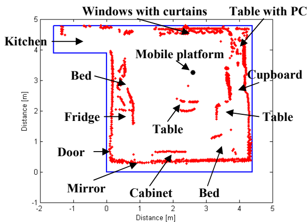
Fig. 12 2D vector map from all measurement points – daylight (top view)
