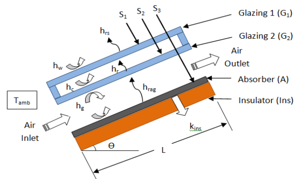
Fig. 2 Physical Model of Double Glazing Solar Collector
