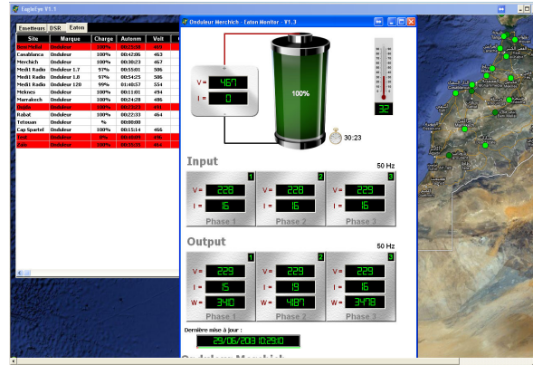
Fig. 4 Example of (inverted variables make Eaton) measurements of equipment device (Power ware 9355-20KVA UPS) after verification of WN by means of RTD
