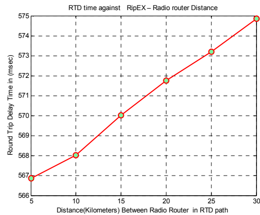
Fig. 6 RTD time against Radio Router Node Distance
