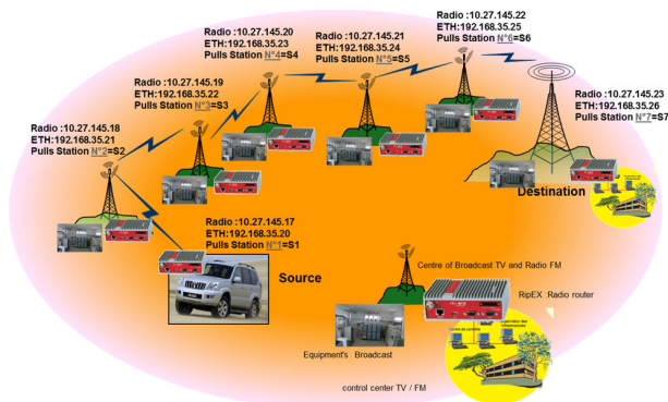
Fig. 5 Network Topologies being studied
