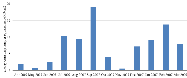
Fig. 10 Energy consumption per unit of the air conditioning system (renewed manufacture)
