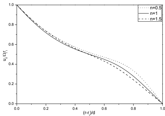
Fig. 2 Variations of the Azimuthal velocity profiles for different fluids for \gamma=0.5 and \Gamma=6 ( Re_i=100 and Re_o=0 )
