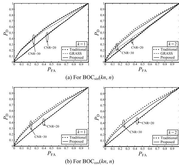
Fig. 5. ROC curves of the proposed, GRASS, and traditional BOC schemes for (a) \text{BOC}_{\sin}(kn, n) and (b) \text{BOC}_{\cos}(kn, n) when k = 1 and 2.
