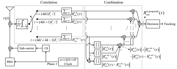
(b) For \text{BOC}_{\cos}(kn, n)
