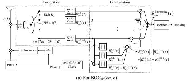
(a) For \text{BOC}_{\sin}(kn, n)
