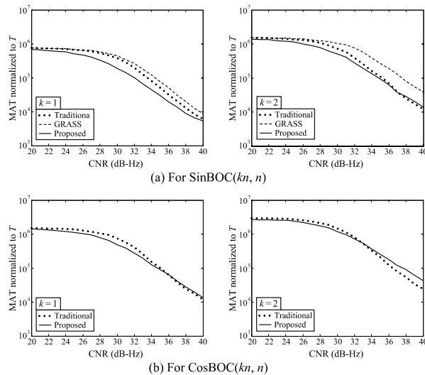
Fig. 6. MAT of the proposed, GRASS, and traditional BOC schemes for (a) \text{BOC}_{\sin}(kn, n) and (b) \text{BOC}_{\cos}(kn, n) when k = 1 and 2.
