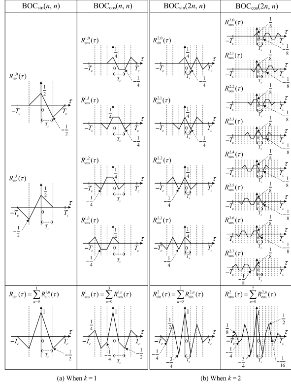
Fig. 1. BOC autocorrelation and the associated sub-correlations when (a) k = 1 and (b) k = 2 in the absence of noise.
