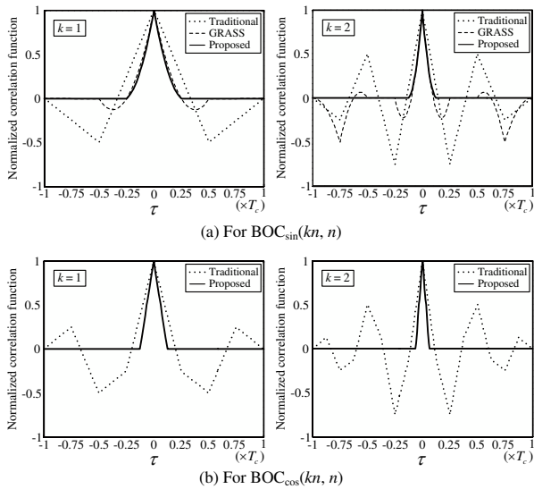
Fig. 4. Normalized correlation functions of the proposed, GRASS, traditional BOC schemes for (a) \text{BOC}_{\sin}(kn, n) and (b) \text{BOC}_{\cos}(kn, n) when k = 1 and 2 in the absence of noise.
