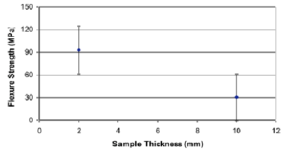
Fig. 6 Effect of sample thickness to flexure strength
