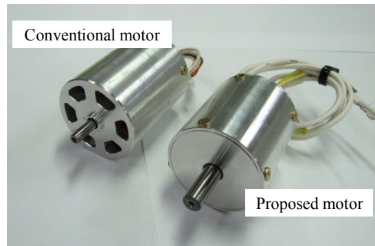
Fig 11 assembled two motors
