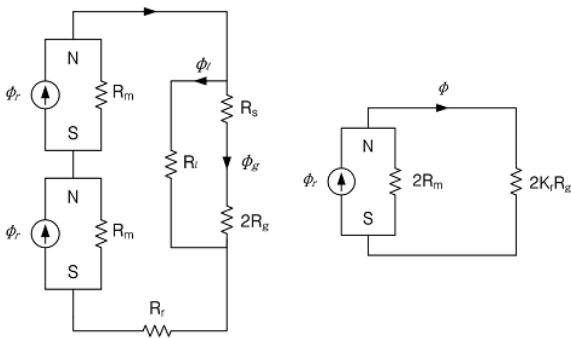
(b) Simplified magnetic circuit
