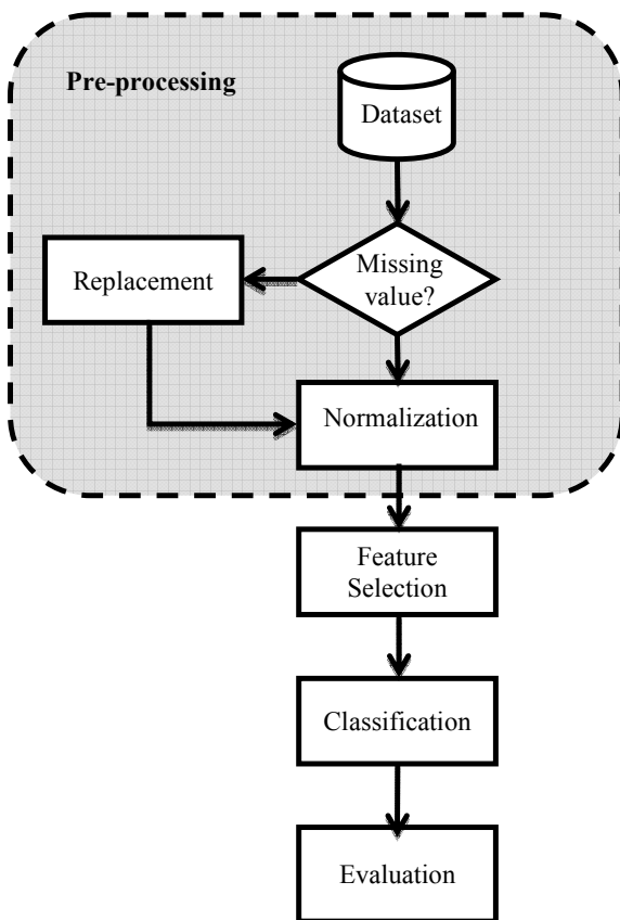
Fig. 1 The data mining procedure of clinical dataset
