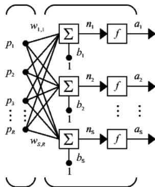
Fig. 3 Network architecture: A single layer of neurons
