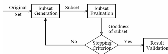
Fig. 1 Steps in Attribute Selection [11]
