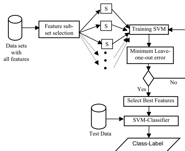
Fig. 3 System Flow with Sequential Backward Feature Selection
