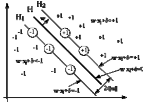
Fig. 1 Optimal hyperplane with maximized margin
